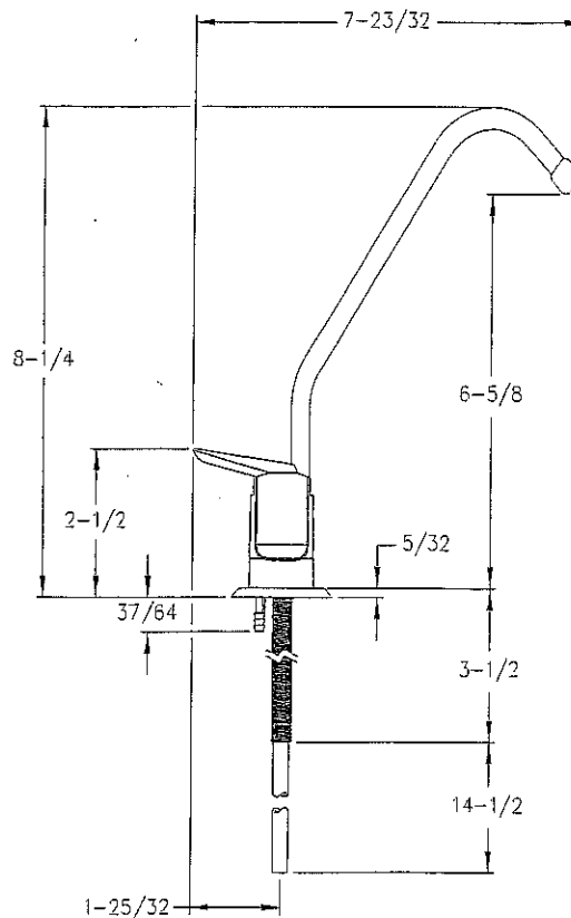
PF500LFBRAG Faucet (with air gap)
